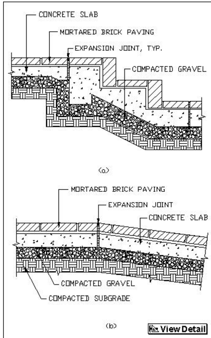
Stair and Ramp Sections
