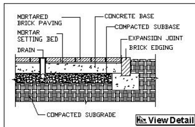
Mortarted Brick Paving
